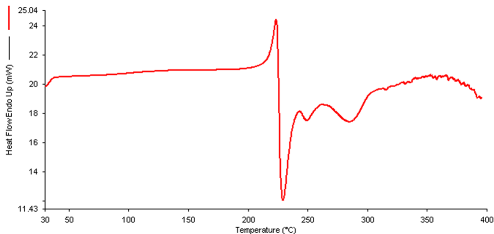
Fig.5: Differential scanning calorimetry of Azilsartan medoxomil
